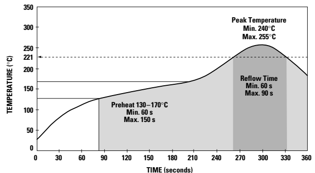
Figure 23. Surface Mount Assembly Temperature Profile.
