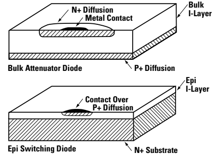
Figure 9. PIN Diode Construction.
