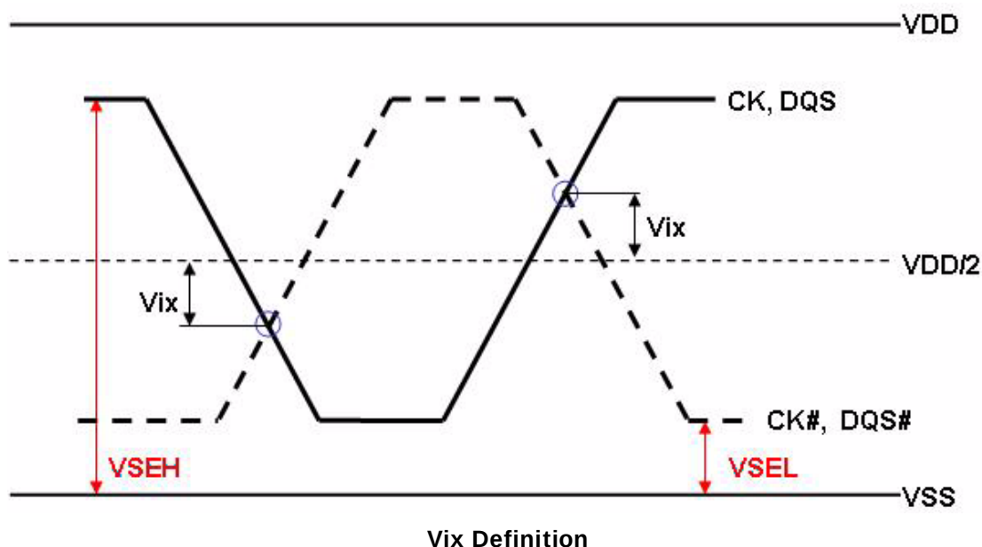
Cross point voltage for differential input signals (CK, DQS)
