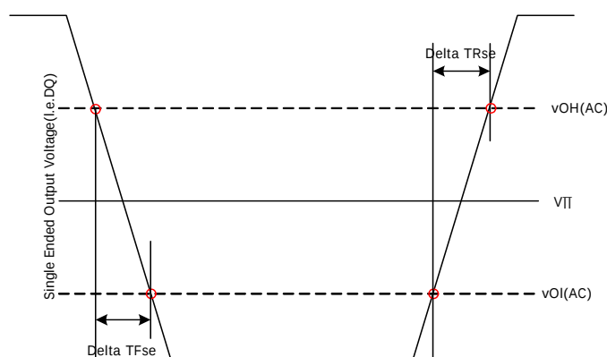
Single Ended Output Slew Rate Definition
