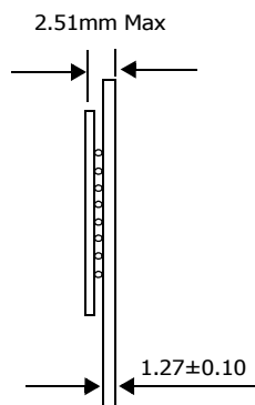
Side
