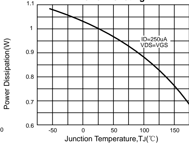
Power De-rating
