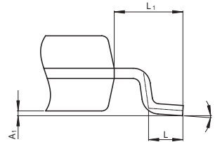
Detail F
