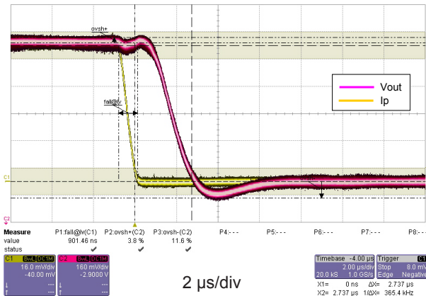
Figure 3: Step response
