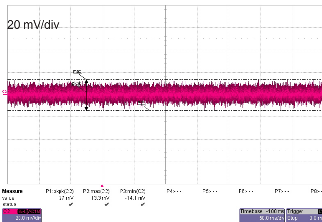
Figure 15: Output noise
