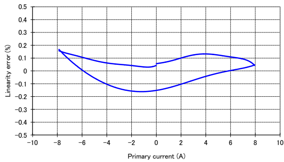
Figure 1: Linearity error
