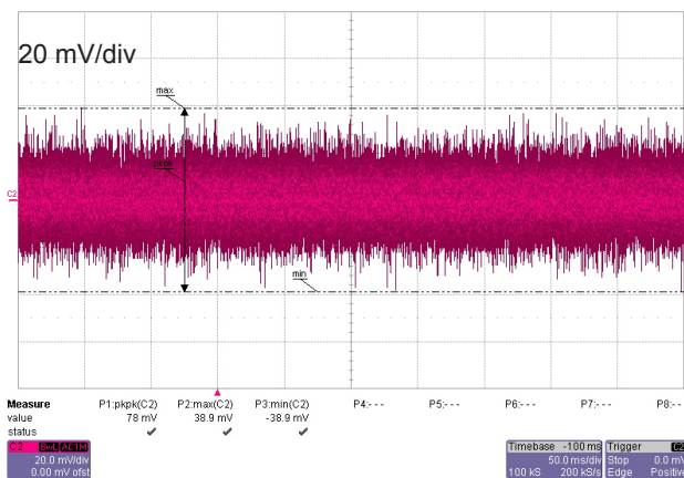
Figure 5: Output noise
