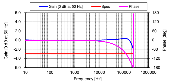
Figure 12: Frequency response
