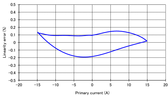
Figure 6: Linearity error
