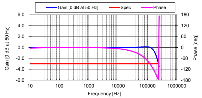
Figure 2: Frequency response
