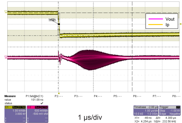
Figure 4: dv/dt
