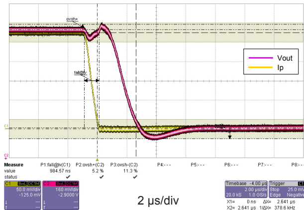
Figure 13: Step response
