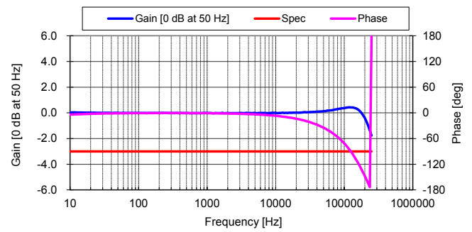
Figure 7: Frequency response
