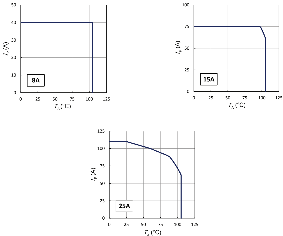
Figure 16: I_p vs T_A for HO series
