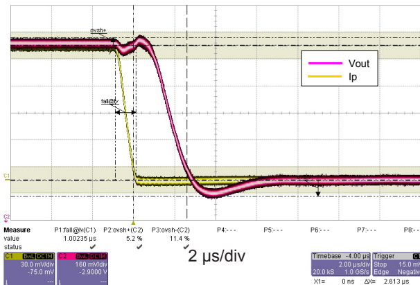
Figure 8: Step response
