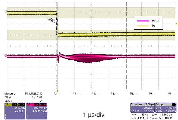
Figure 14: dv/dt
