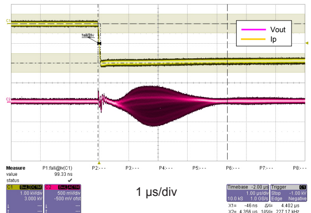
Figure 9: dv/dt
