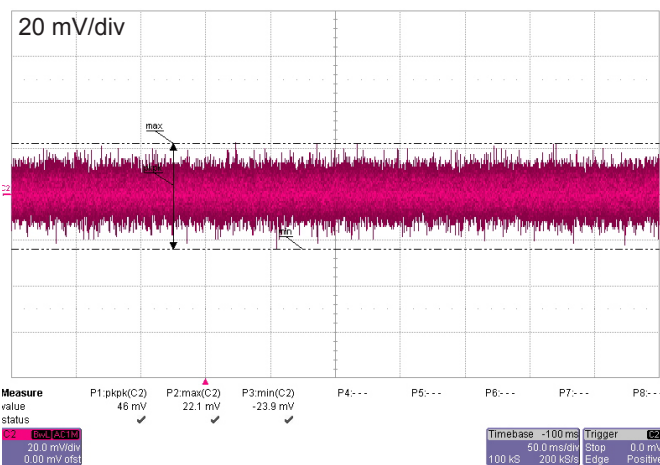
Figure 10: Output noise
