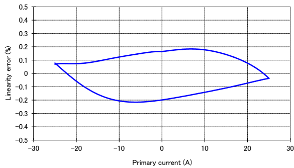
Figure 11: Linearity error
