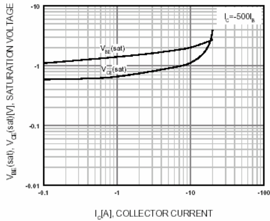
Figure 3. Collector-Emmitter Saturation Voltage Base-Emmitter Saturation Voltage
