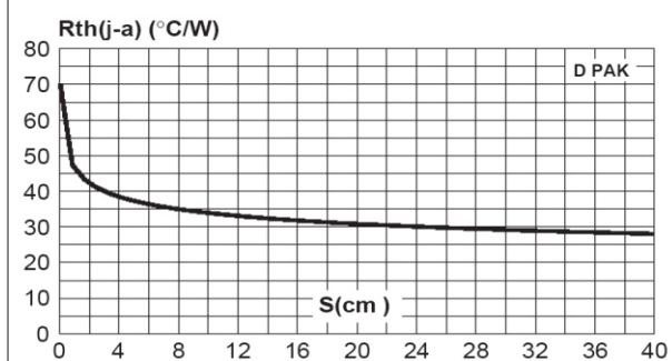
Fig. 10: D PAK Thermal resistance junction to ambient versus copper surface under tab (printed circuit board FR4, copper thickness: 35\text{ }\mu\text{m} ).
