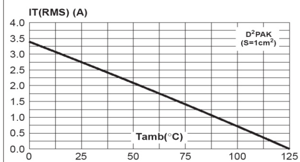
Fig. 2-2: D PAK RMS on-state current versus ambient temperature (printed circuit board FR4, copper thickness: 35 \mu m), full cycle.
