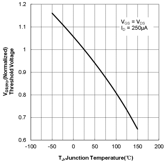
Figure.10 Typical Theshold Voltage vs Junction Temperatur
