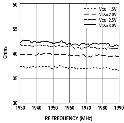
Figure 15A. PCS-CDMA RF Impedance (Real). [1]
