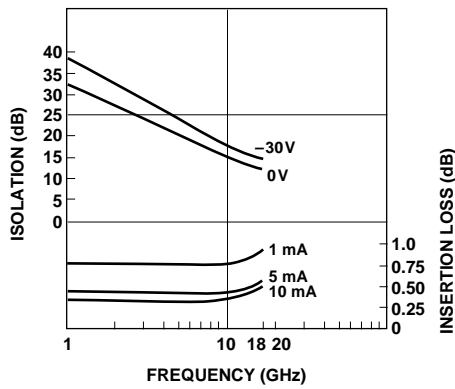
Figure 1. Typical Isolation and Insertion Loss, HPND-4018.
