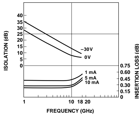
Figure 2. Typical Isolation and Insertion Loss, HPND-4028.
