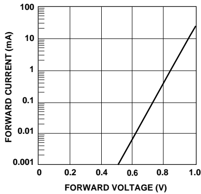
Figure 7. Typical Forward Characteristics.
