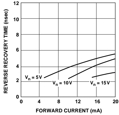
Figure 5. Typical Reverse Recovery Time vs. Forward Current (Series Configuration). HPND-4018.
