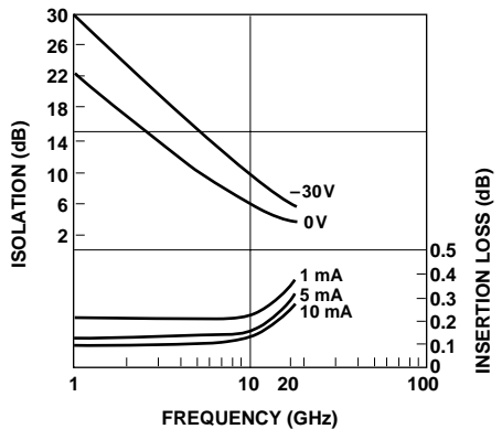
Figure 3. Typical Isolation and Insertion Loss, HPND-4038.
