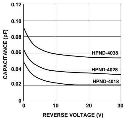
Figure 4. Typical Capacitance vs. Reverse Voltage (at 1 MHz).
