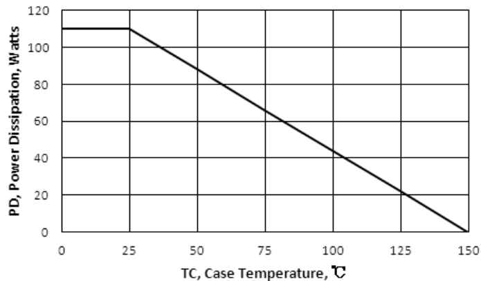
Figure 2 Maximum Power Dissipation vs Case Temperature
