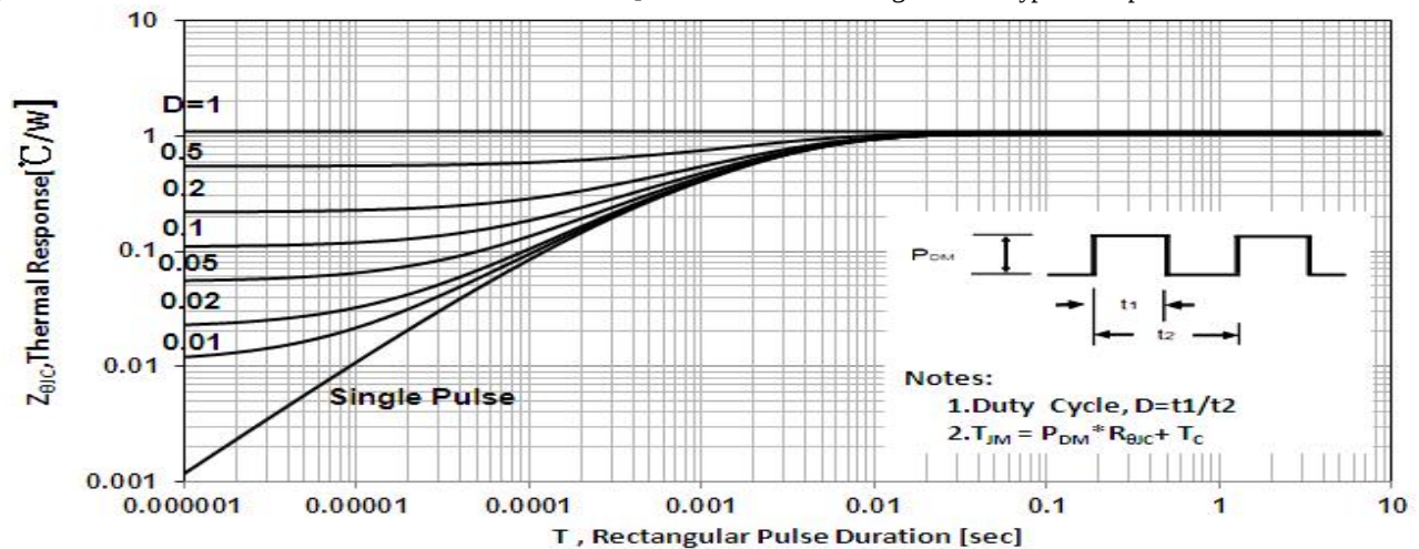
Figure 5 Maximum Rectified Thermal Impedance, Junction to Case
