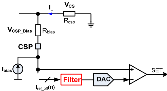
Figure 21: Iref_filter Circuit
