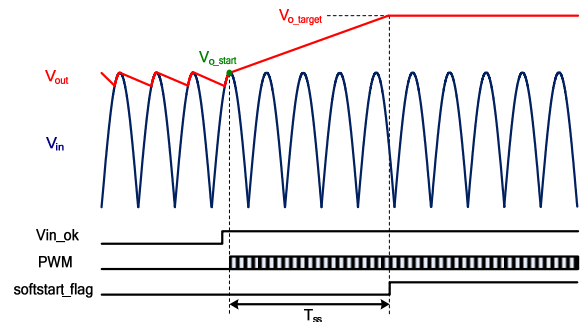
Figure 23: Soft-Start Sequence
