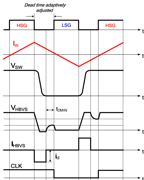
Figure 28: Operation Waveform of ADTA
