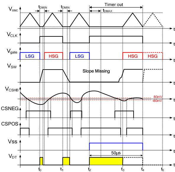
Figure 31: Operating Principle of CMP
