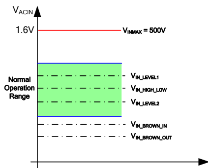
Figure 10: Input Voltage Level for Different Functions
