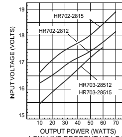
HR702-2812 HR702-2815 HR703-28512 HR703-28515 LOW LINE DROPOUT VS LOAD (50mV DROP) FIGURE 11
