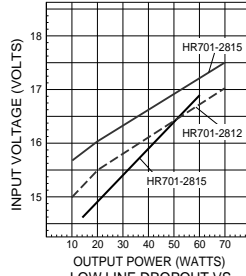
HR701-2815 LOW LINE DROPOUT VS LOAD (50mV DROP) FIGURE 10
