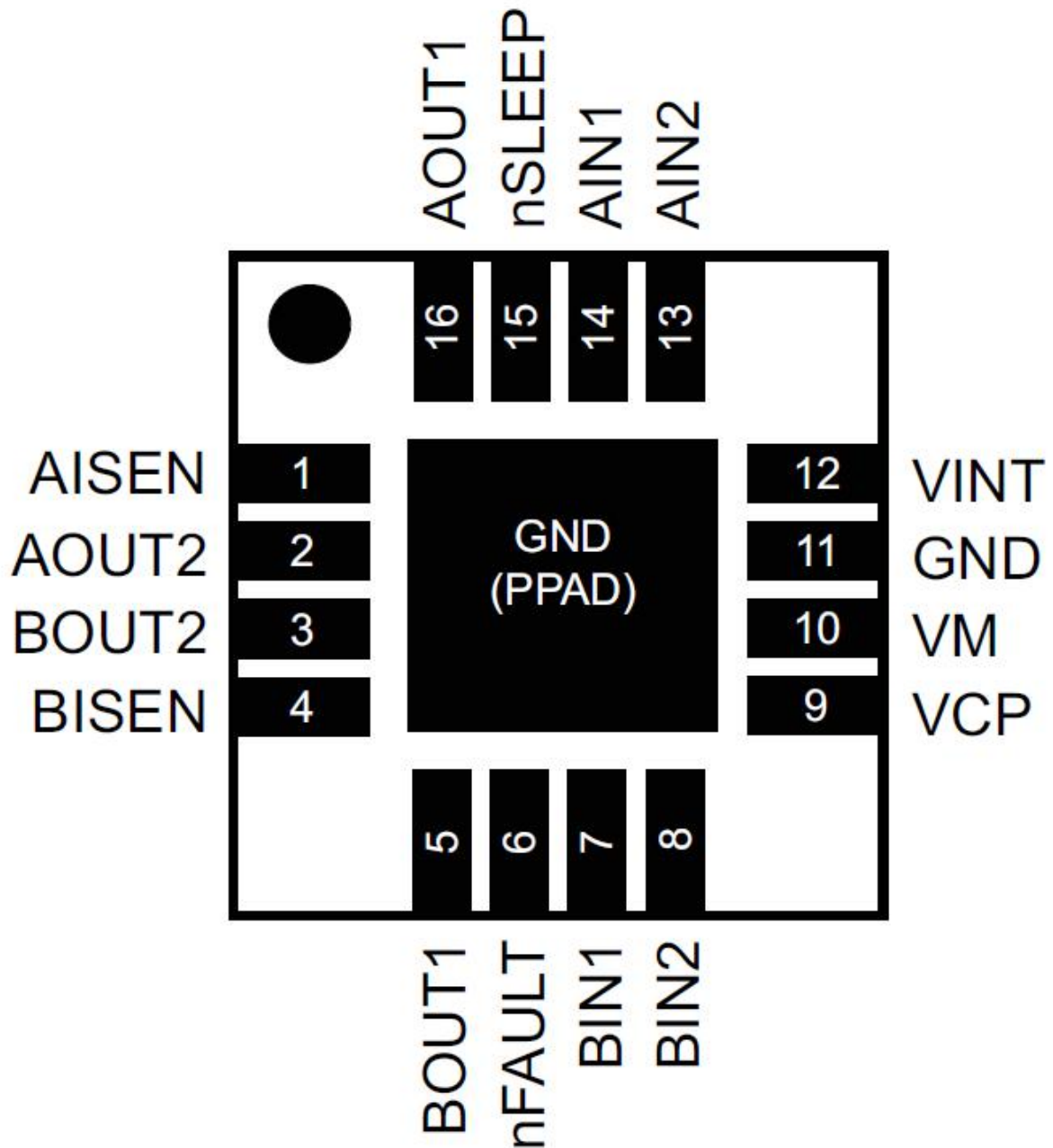
QFN16-PP
