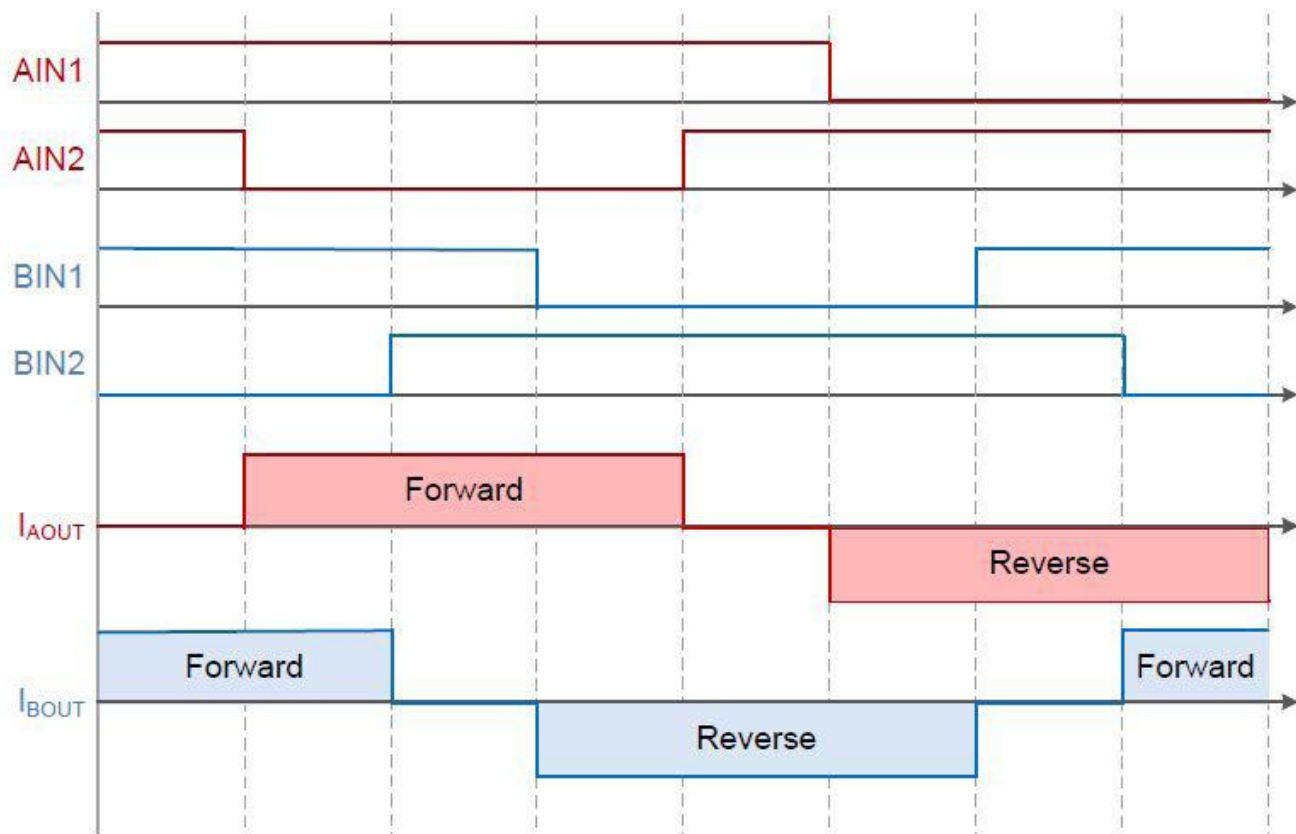
HALF STEP
