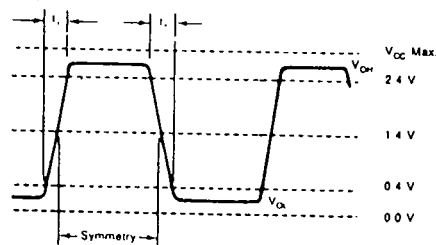
TTL Output Waveform
