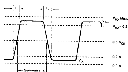
CMOS Output Waveform
