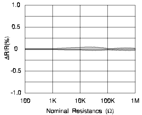
Load Life (Rated Load) (70°C, RCWV 1,000 hrs)
