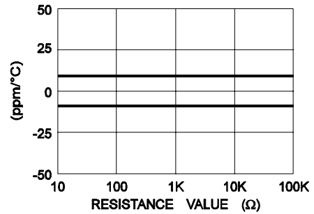
Resistance Temp. Coefficient (25°C/125°C)
