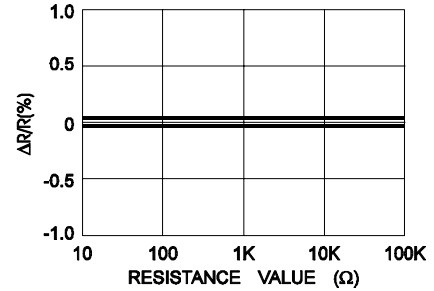
Short-Time Overload
