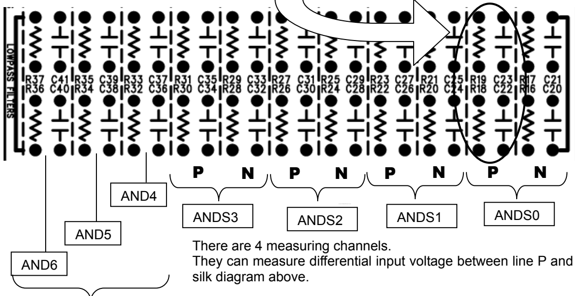
Silk diagram of the low-pass filter
