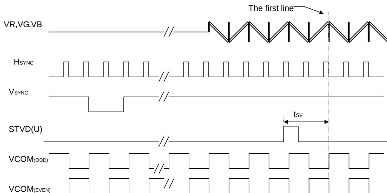
Vertical timing
