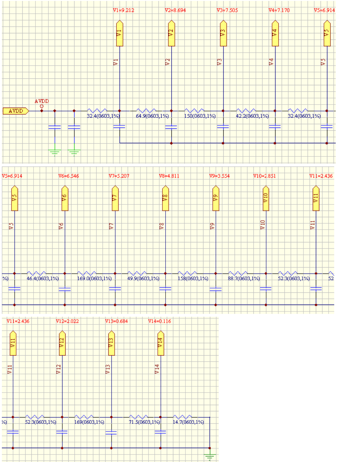
*Suggested Gamma Circuit(AVDD=9.5V).
