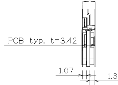
Detail E (2:1)
