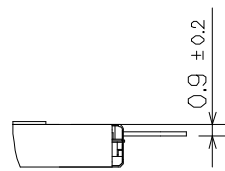
Detail F (2:1)
