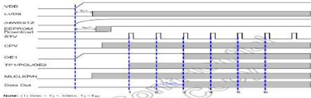
Figure 6.5: Power up sequence
