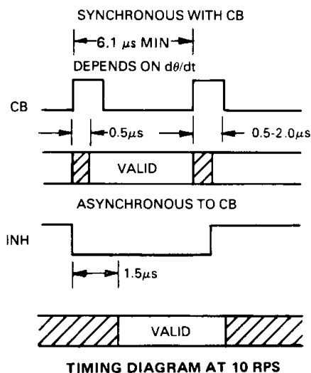
TIMING DIAGRAM AT 10 RPS
