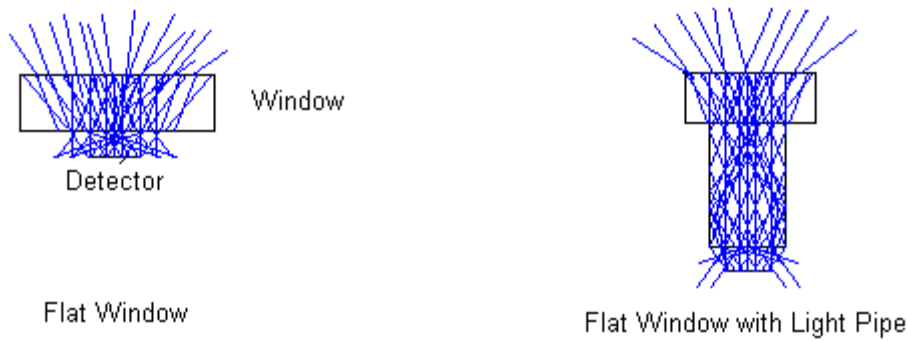
Figure 12. Recommended window design.
