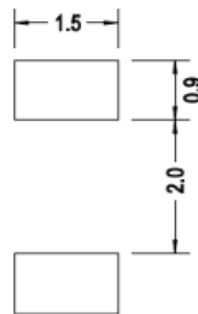
Figure 6: Recommended Soldering Land Pattern
