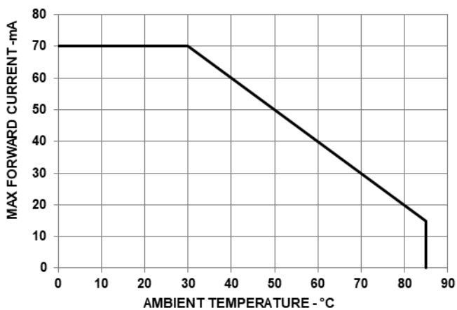
Figure 5: Derating Curve
