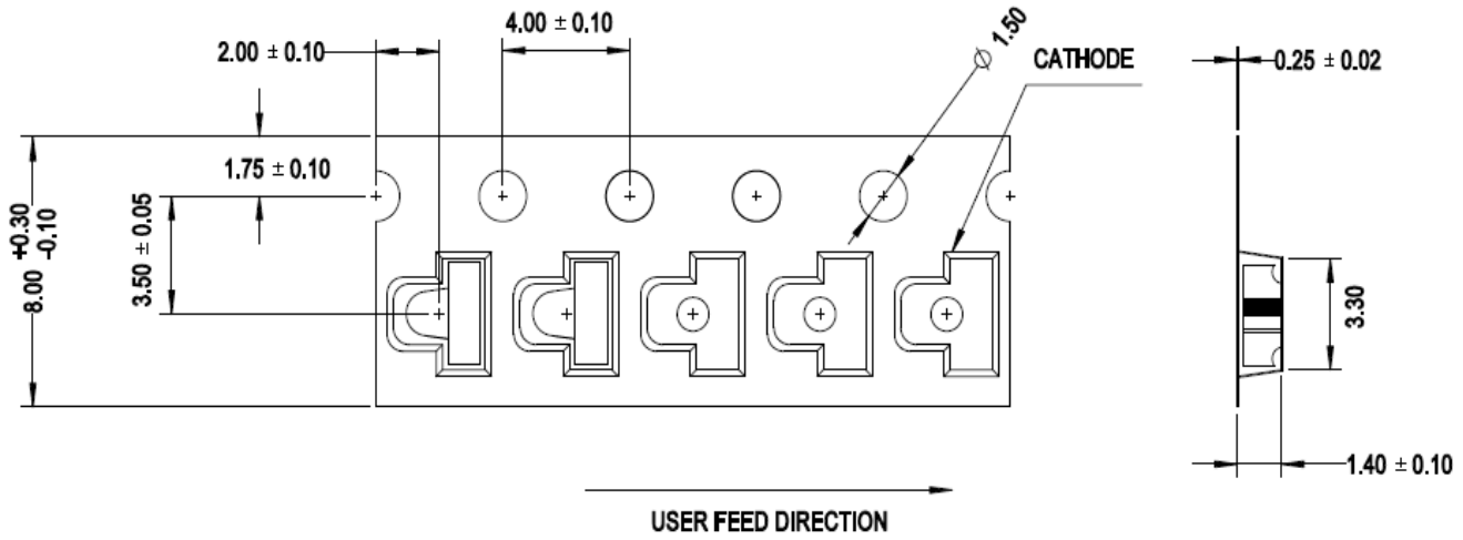
Figure 7: Carrier Tape Dimensions
