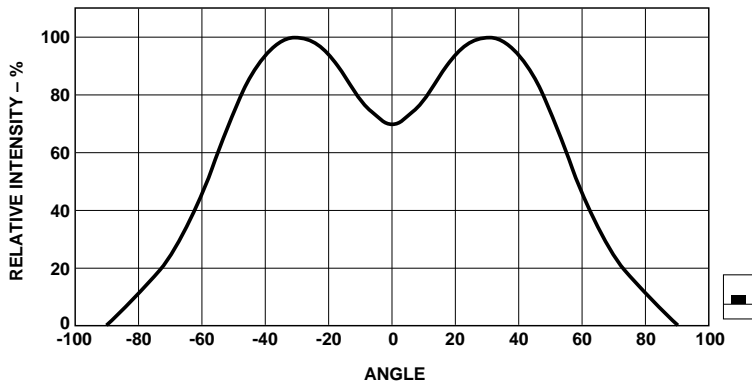
Figure 5c. Relative intensity vs. angle for HSMx-C110.
