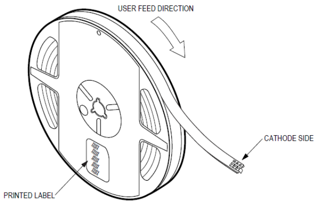
Figure 7. Reel orientation
