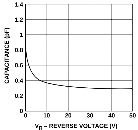
Figure 2. Capacitance vs Reverse Voltage.
