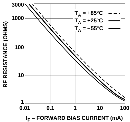
Figure 1. RF Resistance vs Forward Bias Current
