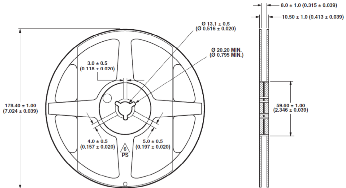
Figure 13. Reel dimensions
