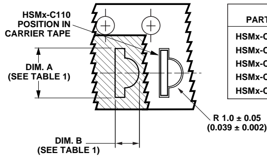
Figure 15. Tape dimensions.
