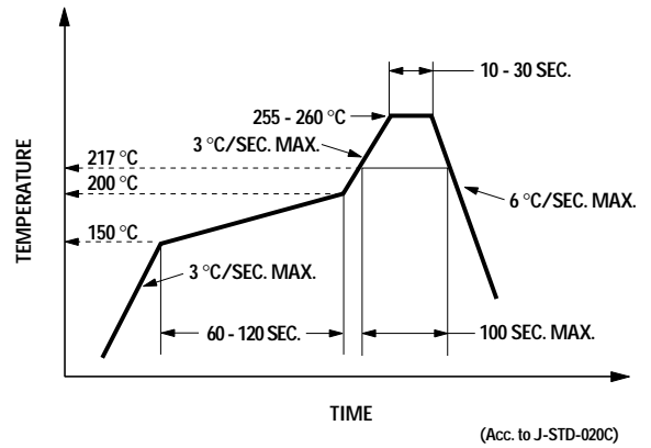
Figure 8. Recommended Pb-free reflow soldering profile.
