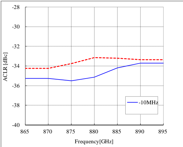
ACLR vs. Frequency
