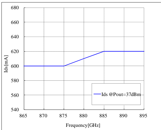
Total Ids vs. Frequency
