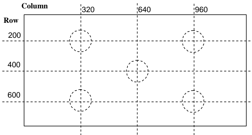
Figure 2. White Luminance and Uniformity Measurement Locations (5 points)
