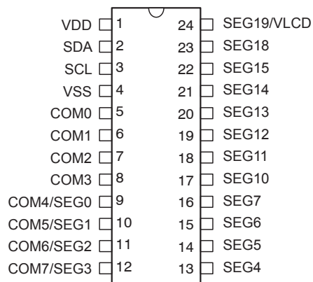
HT16C21 24 SOP-A
