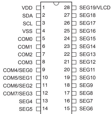
HT16C21 28 SOP-A
