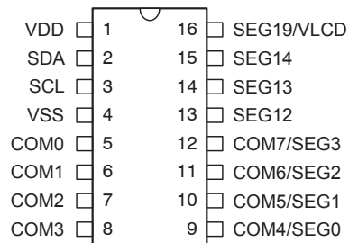
HT16C21 16 NSOP-A
