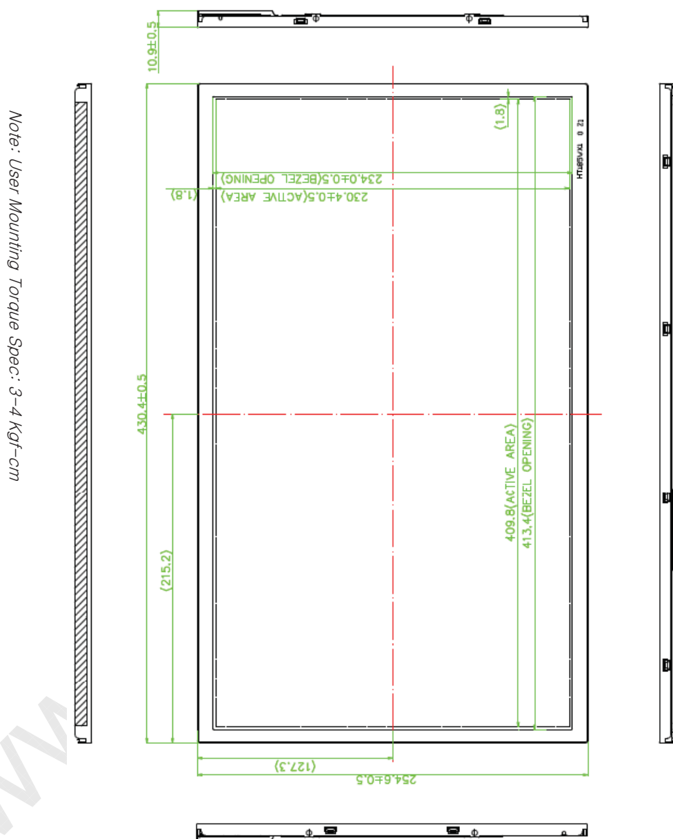
Figure 5. TFT-LCD Module Outline Dimensions (Front view)
