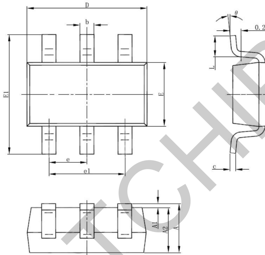
SOT23-6 Package Outline Dimensions
