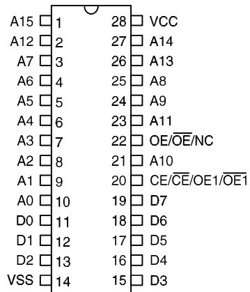
HT23C512 - 28 DIP/SOP
