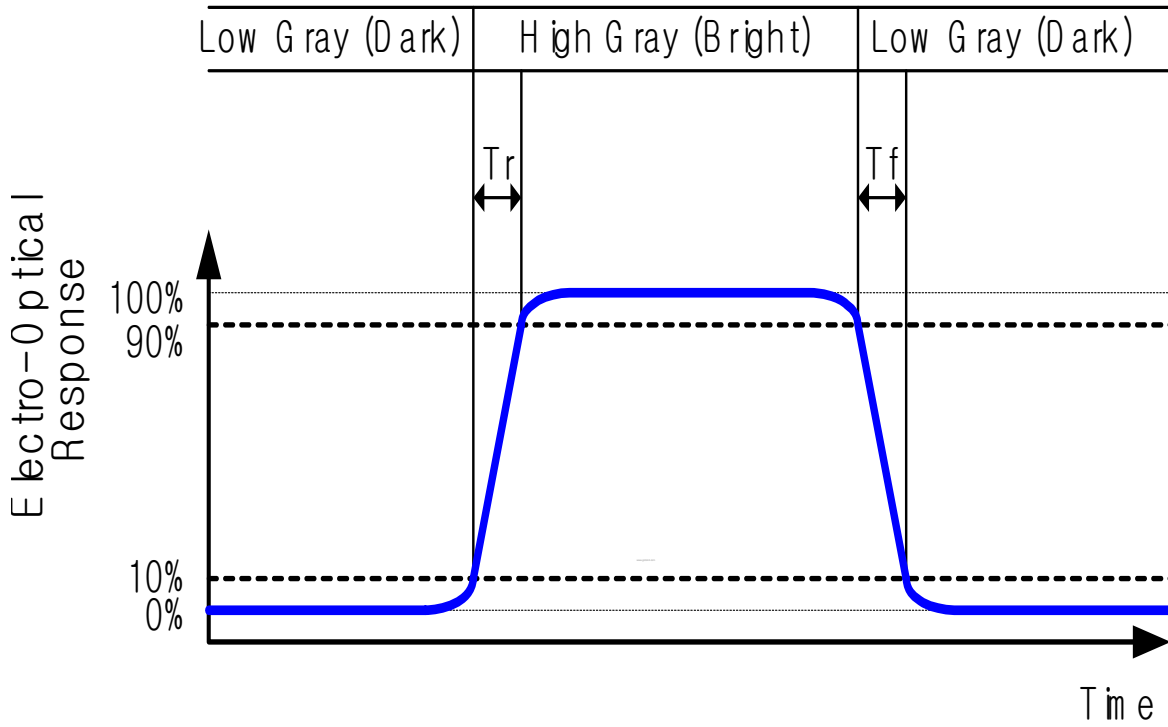
Figure 2. Response Time Testing
