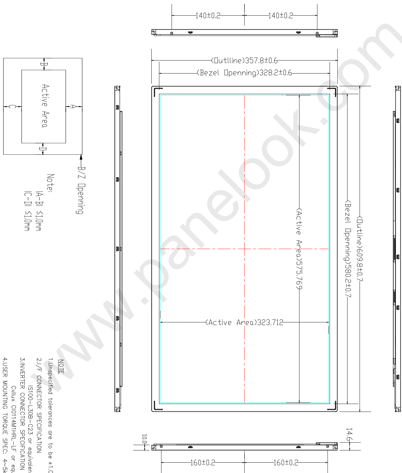
Figure 4. TFT-LCD Module Outline Dimensions (Front view)
