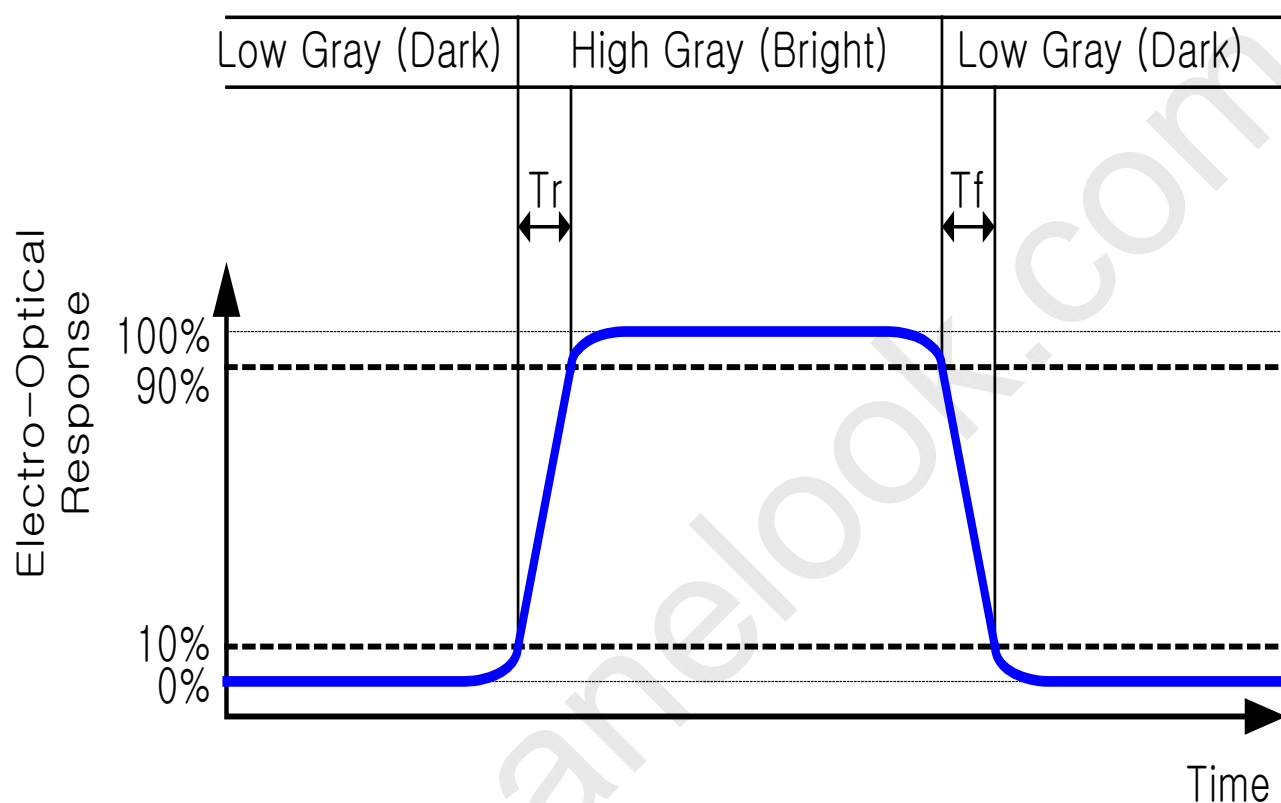
Figure 3. Response Time Testing
