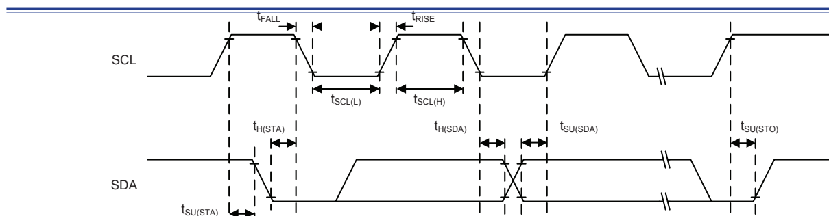
Figure 8. I 2 C Timing Diagrams
