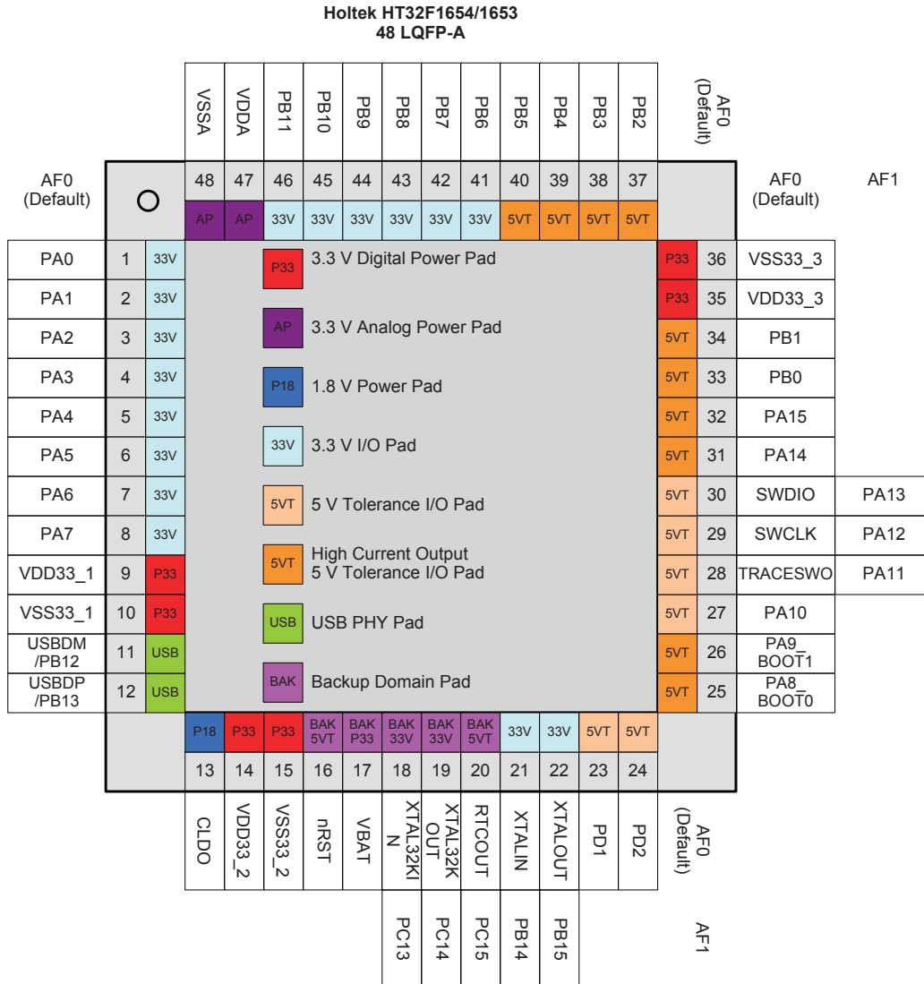
Figure 4 HT32F1654/1653 LQFP-48 Pin Assignment
