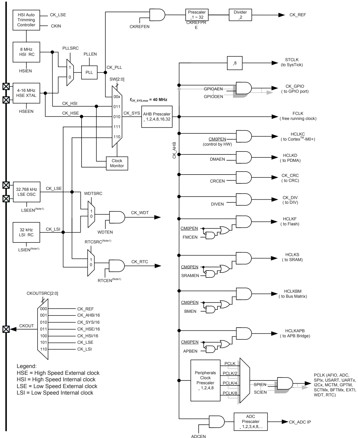
Figure 3. Clock Structure
