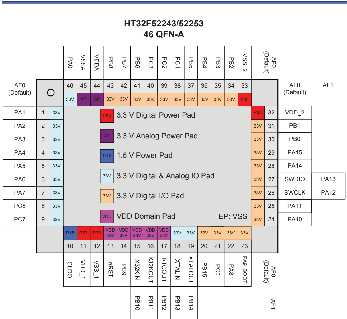
Figure 5. HT32F52243/52253 46-pin QFN Pin Assignment
