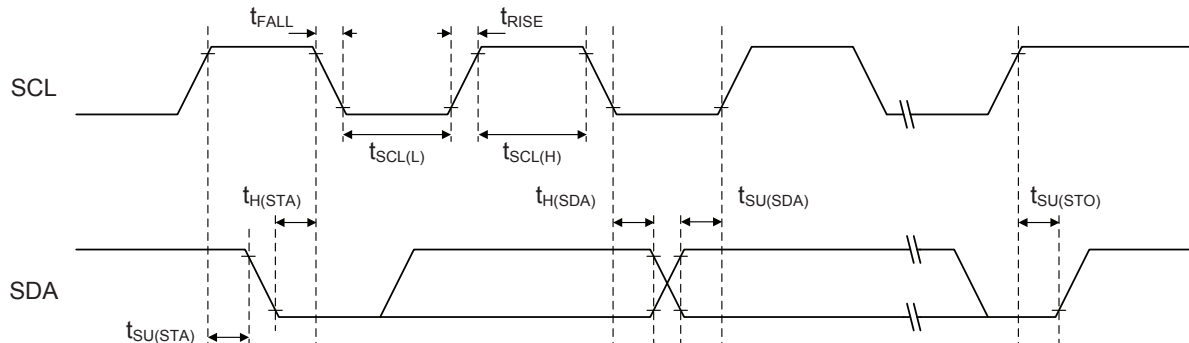
Figure 9. I 2 C Timing Diagrams
