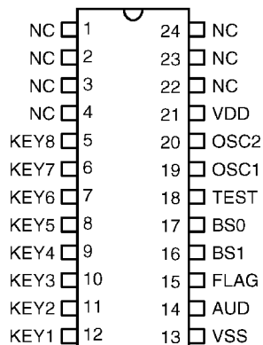
HT3864 – 24 DIP/SOP
