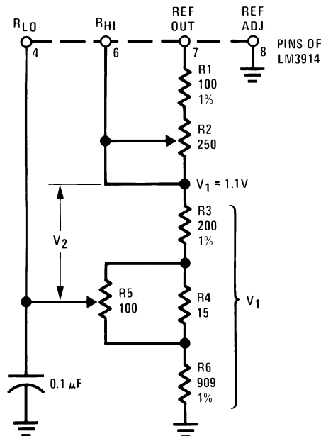
Figure 25. Greatly Expanded Scale (Bar Mode Only)
