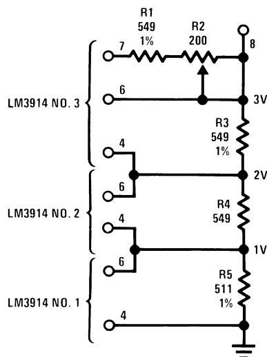
Figure 27. Adjusting Linearity of Several Stacked Dividers
