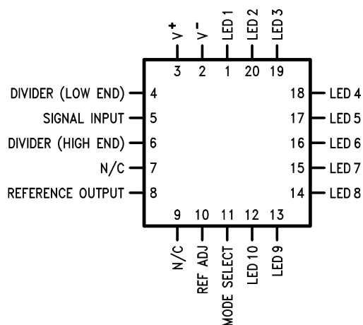
Figure 28. PLCC20
