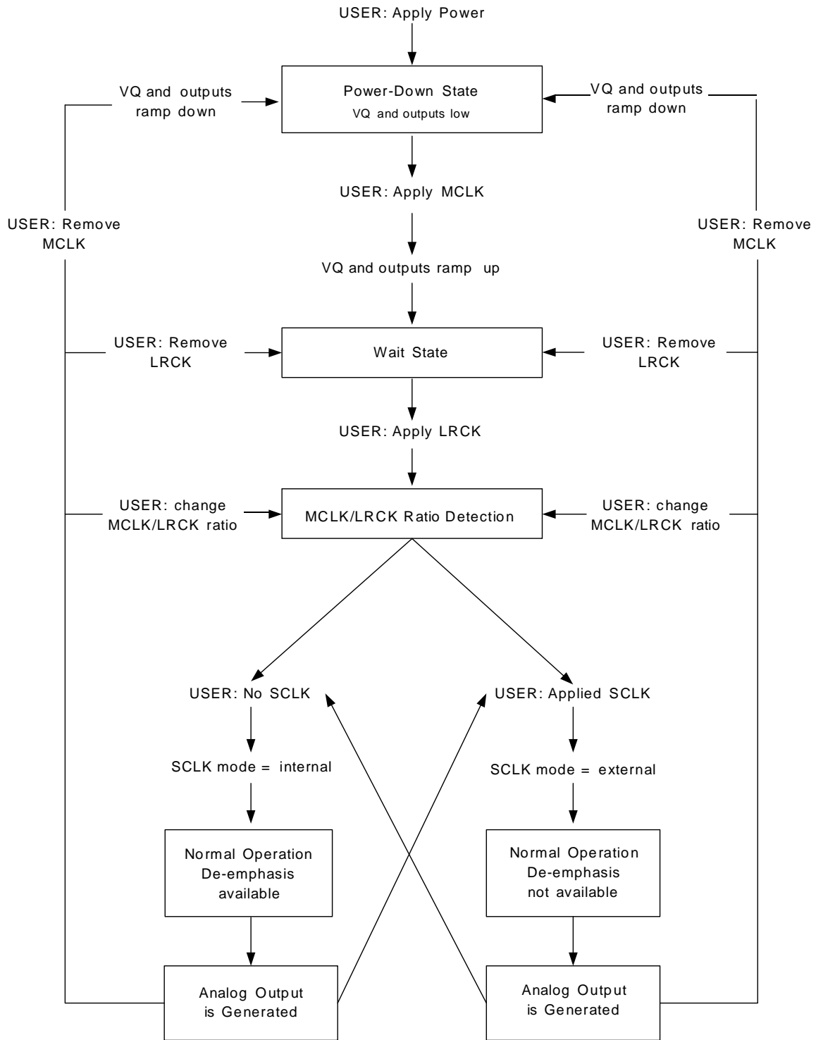
Figure 12. HT4344/5/6/8 Initialization and Power-Down Sequence
