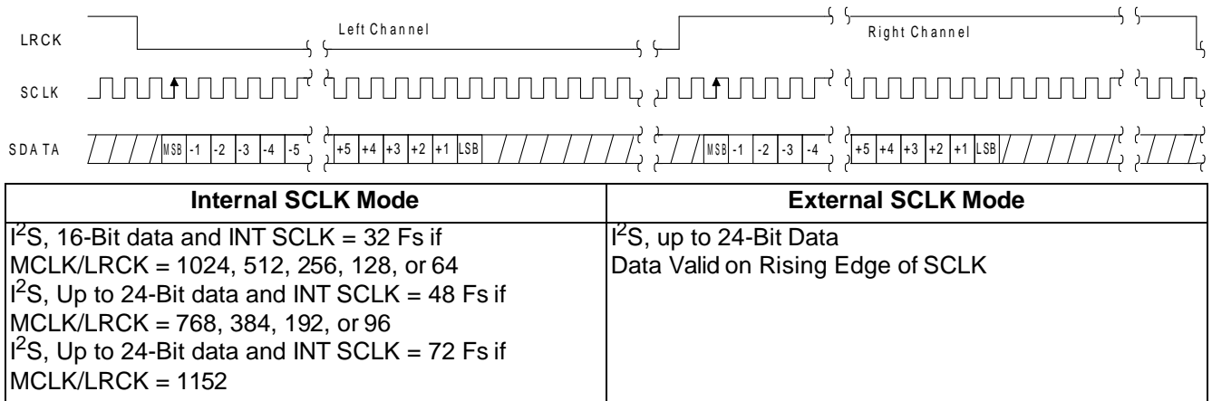
Figure 7. HT4344 Data Format (I 2 S)
