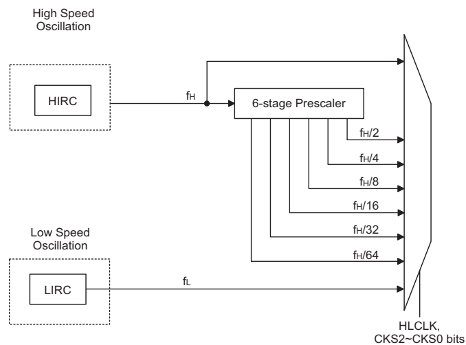
System Clock Configurations
