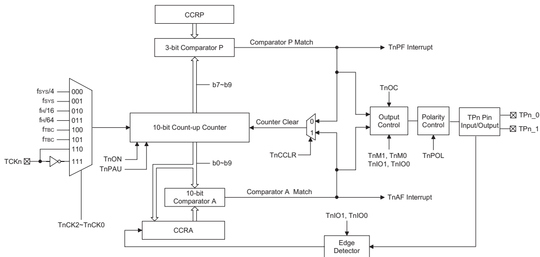
Standard Type TM Block Diagram (n=0)
