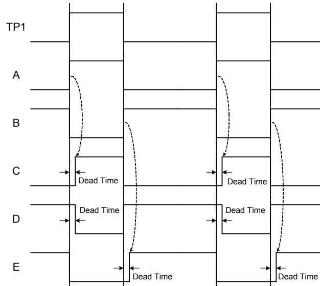
Complementary PWM Output Waveform
