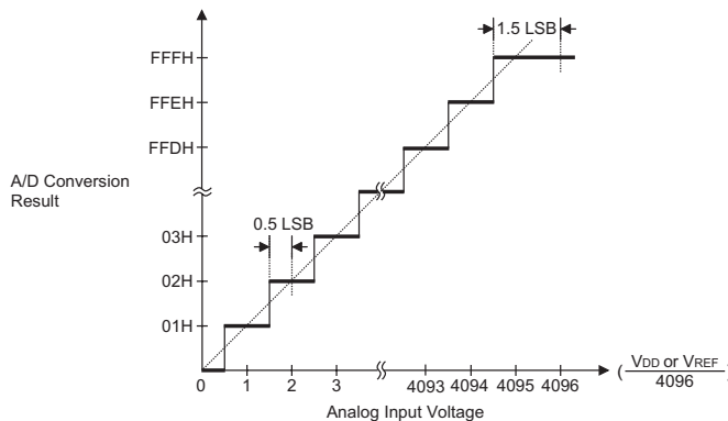
Ideal A/D Transfer Function
