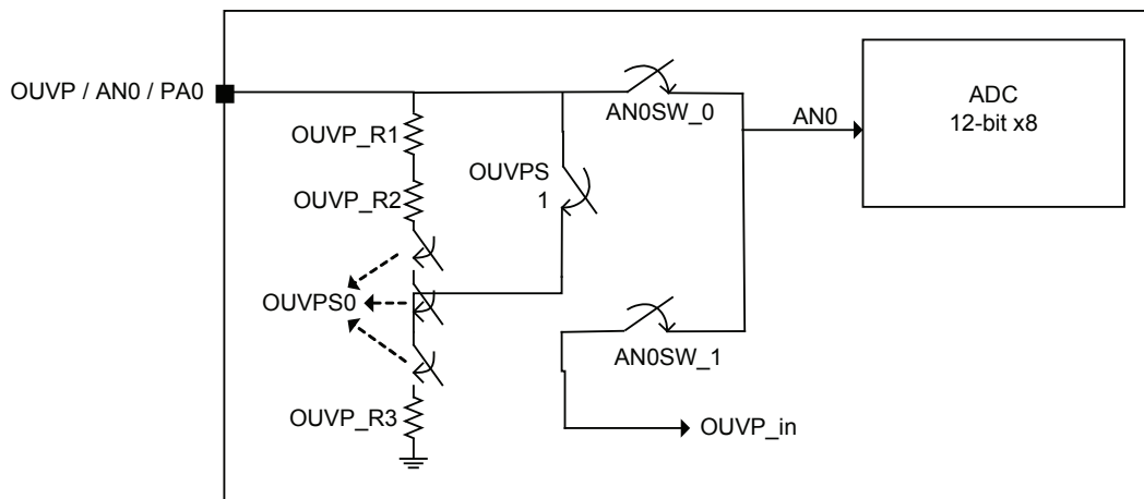
OUVP Pin internal Divider Resistor and Switch Circuit
