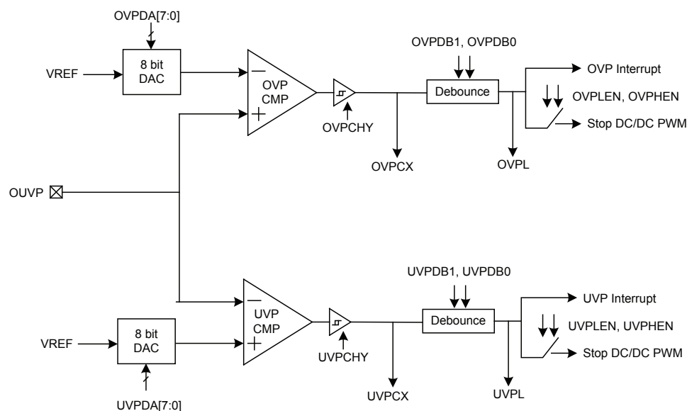
OUPV Protection Block Diagram
