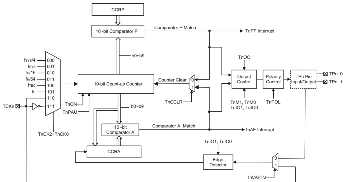
Periodic Type TM Block Diagram (n=1)
