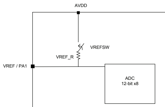
VREF Pin internal Divider Resistor and Switch Circuit
