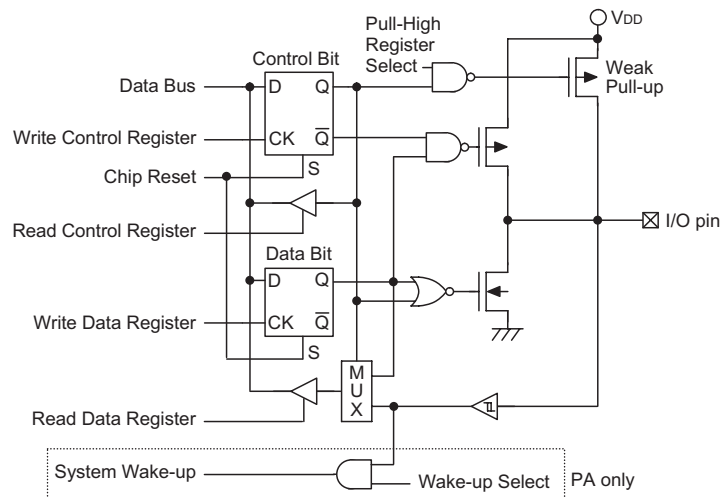
PA/PC/PB0/PB2/PB4 Input/Output Structure
