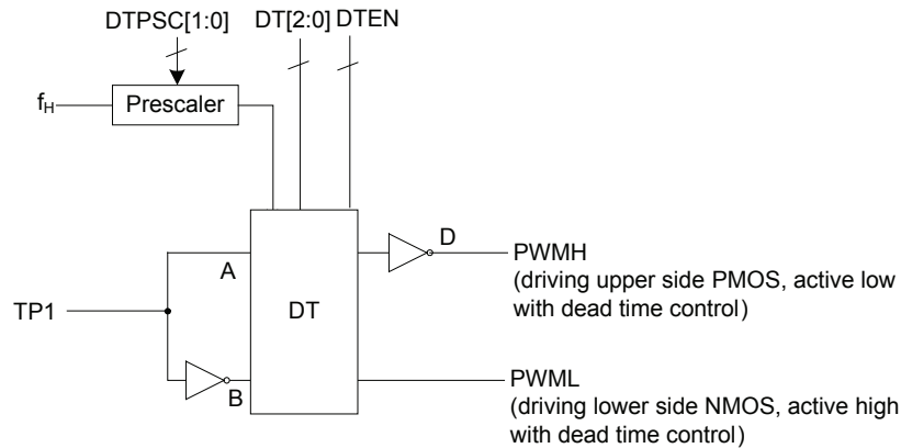
Complementary PWM Output Block Diagram
