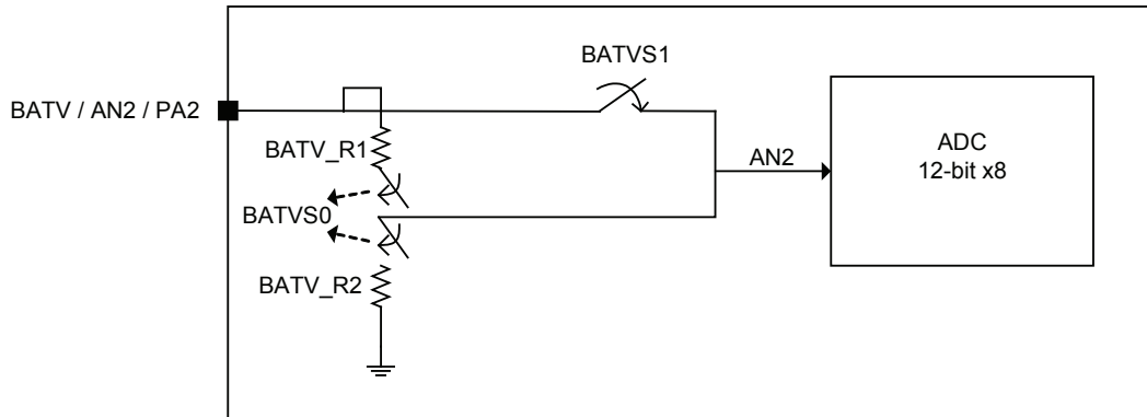
BATV Pin internal Divider Resistor and Switch Circuit
