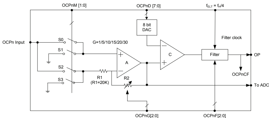
Over Current Protection Block Diagram
