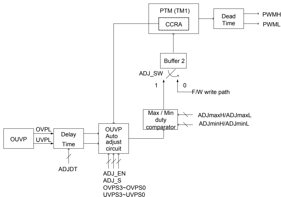
Auto-adjust DC-DC Block Diagram
