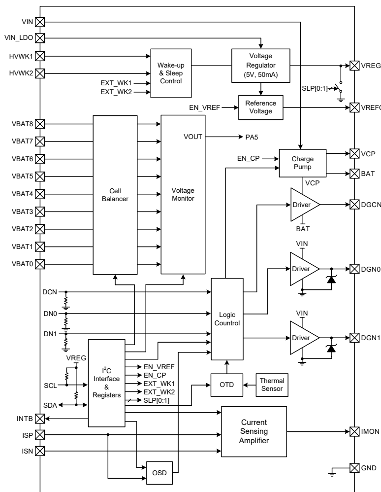
Individual Cell Voltage Monitor Block Diagram
