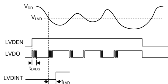
LVD Operation
