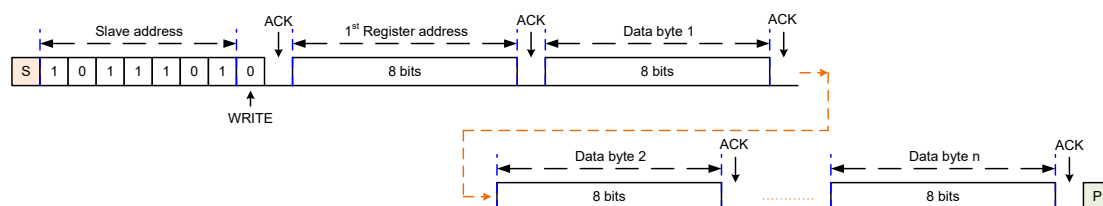
Multiple Data Bytes Write Sequence:
