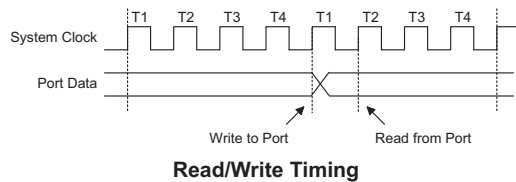
Read/Write Timing
