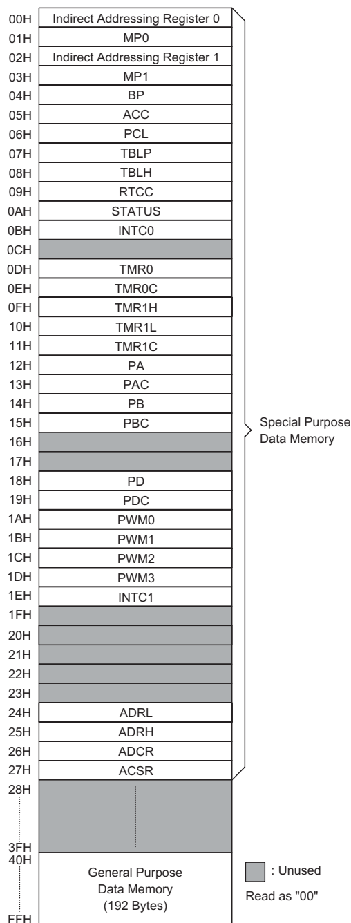
RAM Mapping
